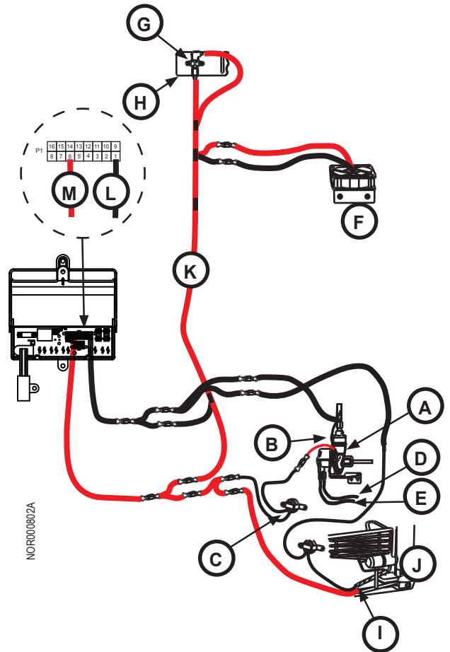
Fig. 23 - Ice maker, fan, and cold weather heater wiring
