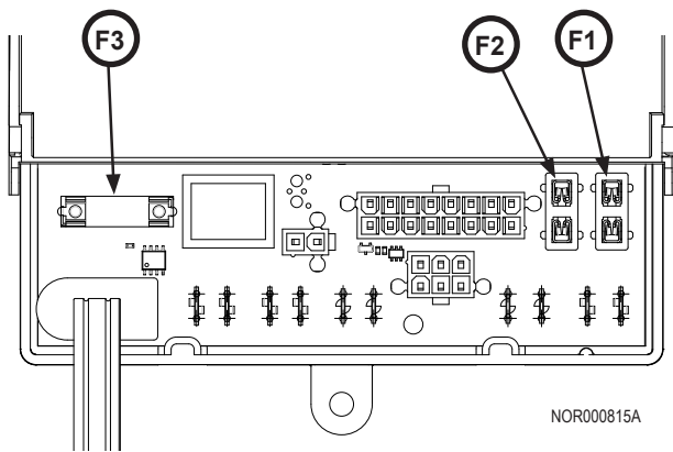
Fig. 7 - Fuse locations
