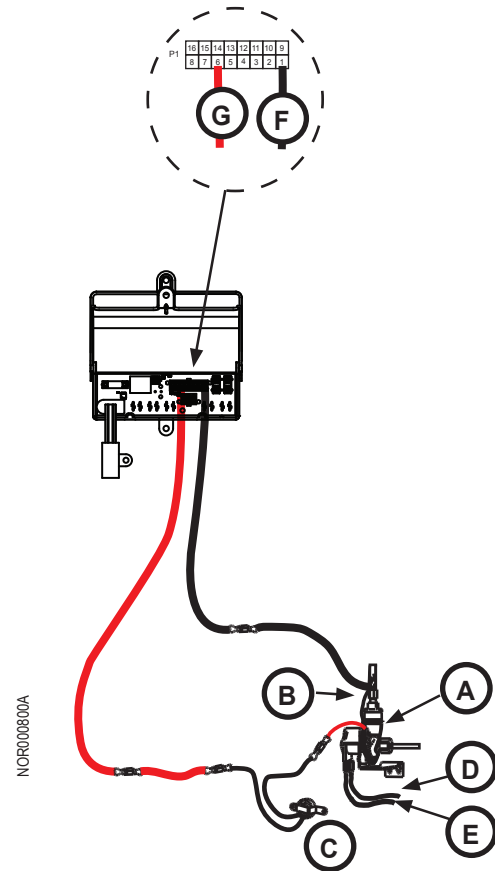
Fig. 21 - Ice maker only wiring
